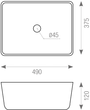
187757 Lavabo Wonder Silver 49×37,5×12 cm./19.3"×14.8"×4.7" E450
