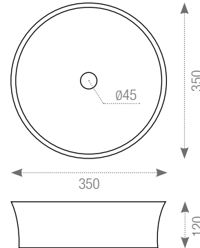
188621 Lavabo Terrazo 35×35×12 cm./13.8"×13.8"×4.7" E800
